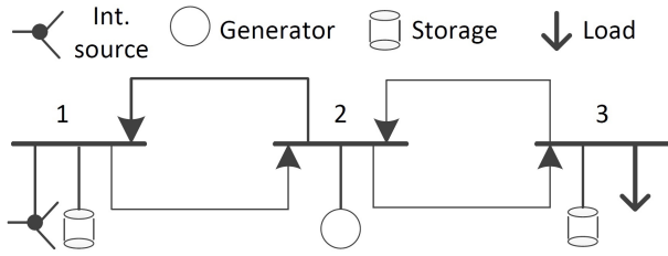
Fig. 3. The 3-bus test network of the case study. Network comprises of an intermittent source, two storage devices, a consumer with a given power load, and a generator. Branch arrows indicate power flow directions.
