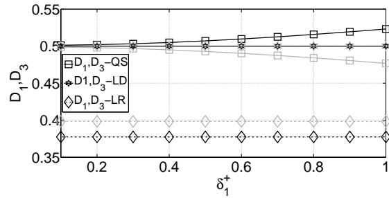
Fig. 5. Storage policies of devices at node 1 ( D_1 , dark line) and node 3 ( D_3 , light line) for different uncertainty levels \delta_1^+ . Plot contains POPF solution corresponding to the QS model (square), the LR model (diamond), and the LD model (star). Figure illustrates the QS model consistency with B1 and the LR model consistency with B2.
