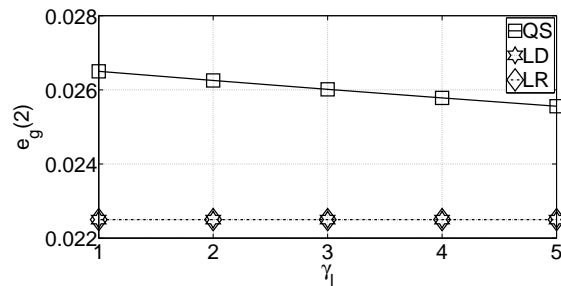
Fig. 6. Generator output e_g(2) at different loss penalties \Gamma_l . Plot contains POPF solution corresponding to the QS model (square), the LR model (diamond), and the LD model (star).
