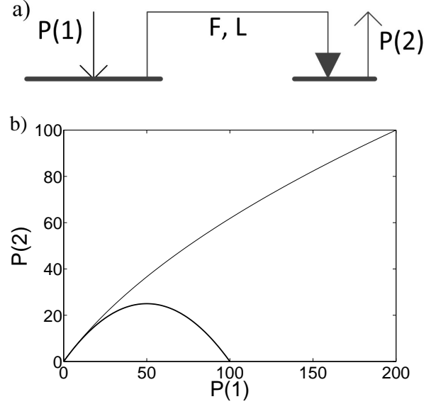
Fig. 1. Example illustrating 2 means of integrating losses into \ell -POPF. (a) Example 2-node network where P(1) > 0 and P(2) > 0 . Arrows indicate power flow directions. (b) Power transmitted P(2) as a function of power injected P(1) when losses are subtracted from incoming flows (heavy line) or added to outgoing flows (light line). Subtraction from incoming flows yields limited maximum power transfer.
